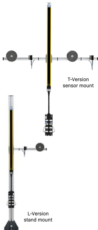
2 sensors - 1 directional muting MUT-SET-L-01, MUT-SET-L-02
